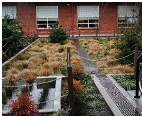
Figure 18.12 Bioretention system inundated during heavy rain, showing submerged forebay (front left), Portland, Oregon (courtesy Environmental Services, City of Portland)
