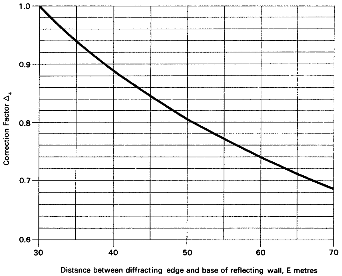
Chart 14 CORRECTION FACTOR \Delta_4 IN TERMS OF DISTANCE, E. [To be used in conjunction with Charts 13 and 15]
