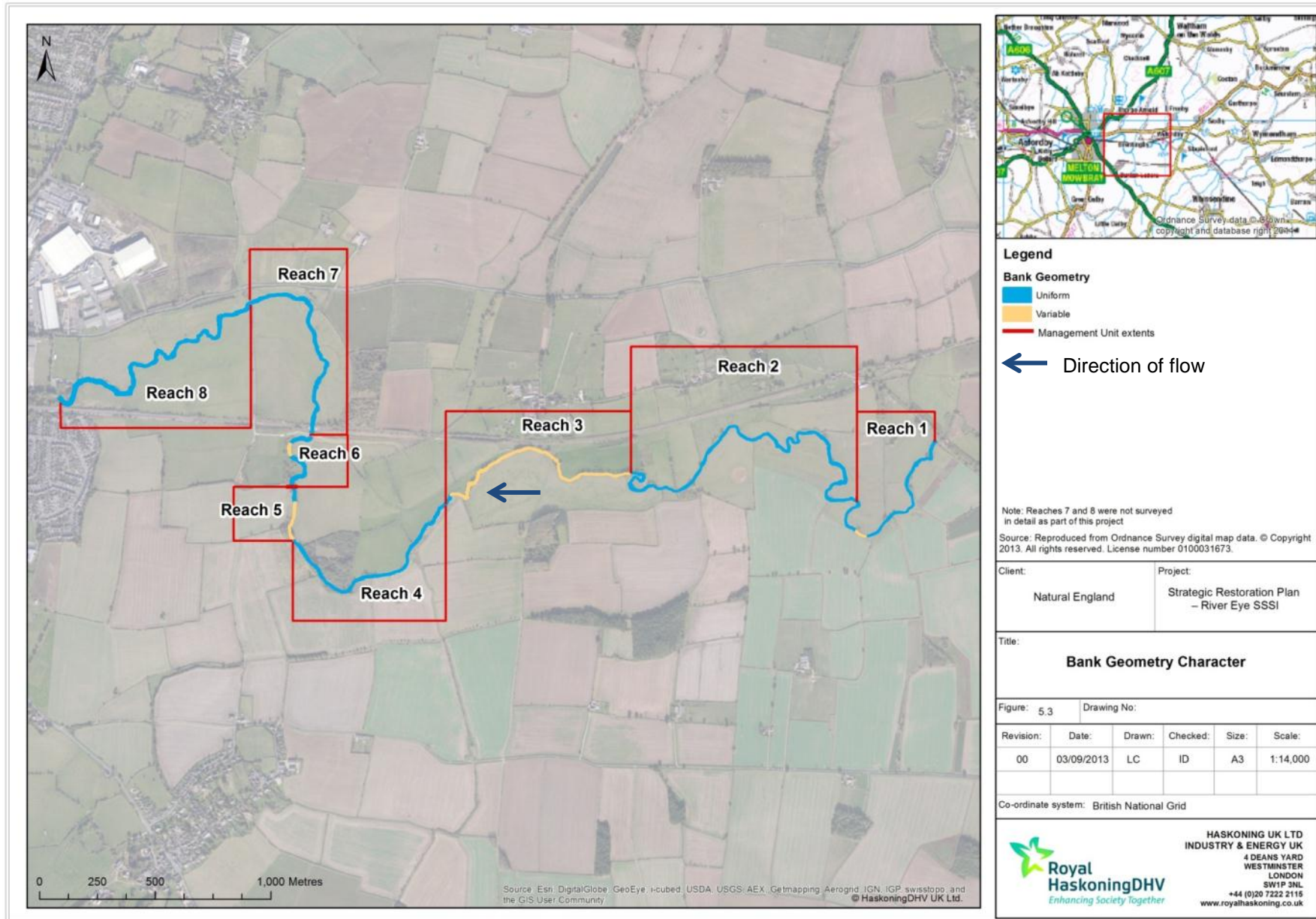
Figure 5.3: Bank geometry character overview
