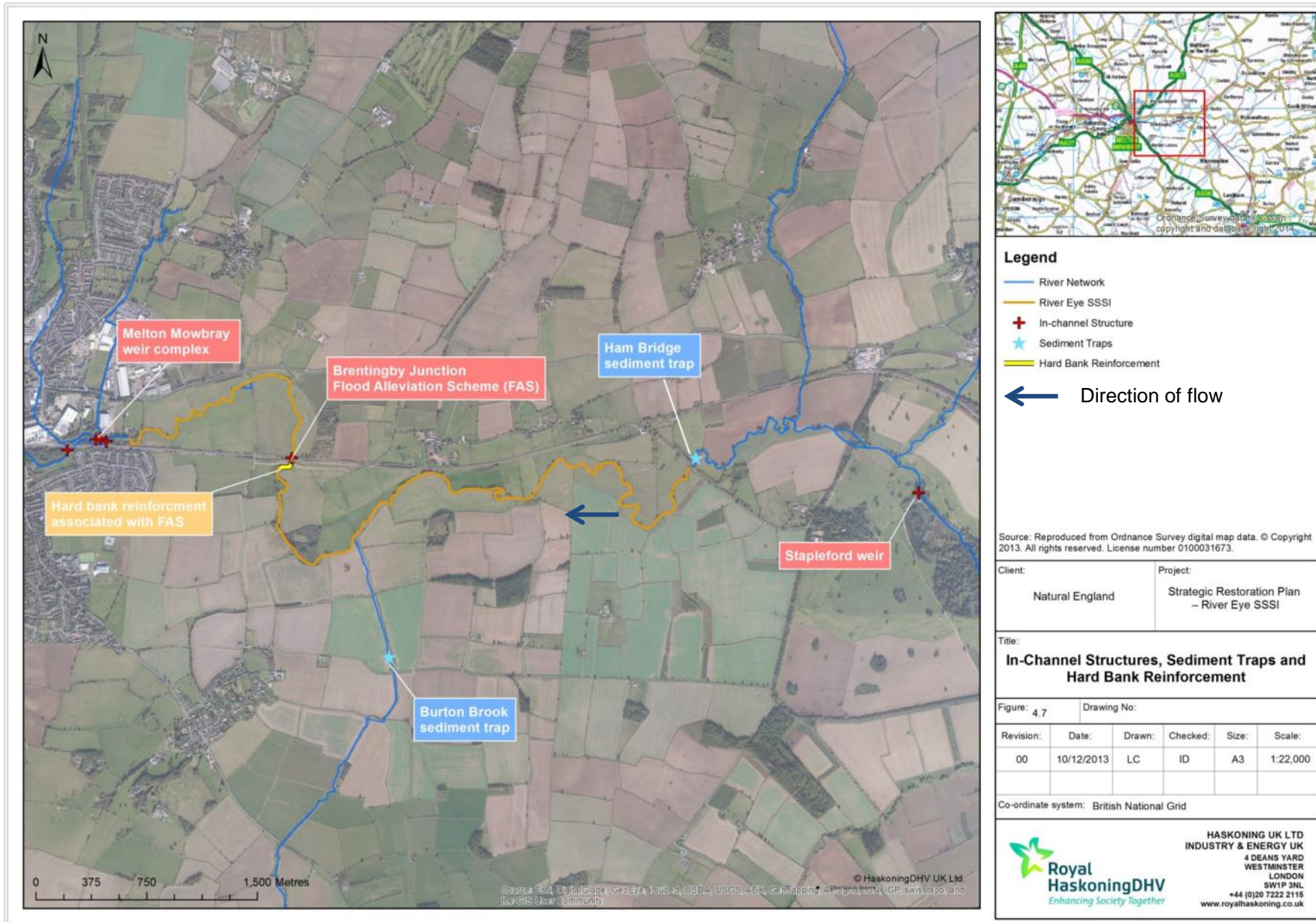
Figure 4.7: In-channel structures in the River Eye catchment
