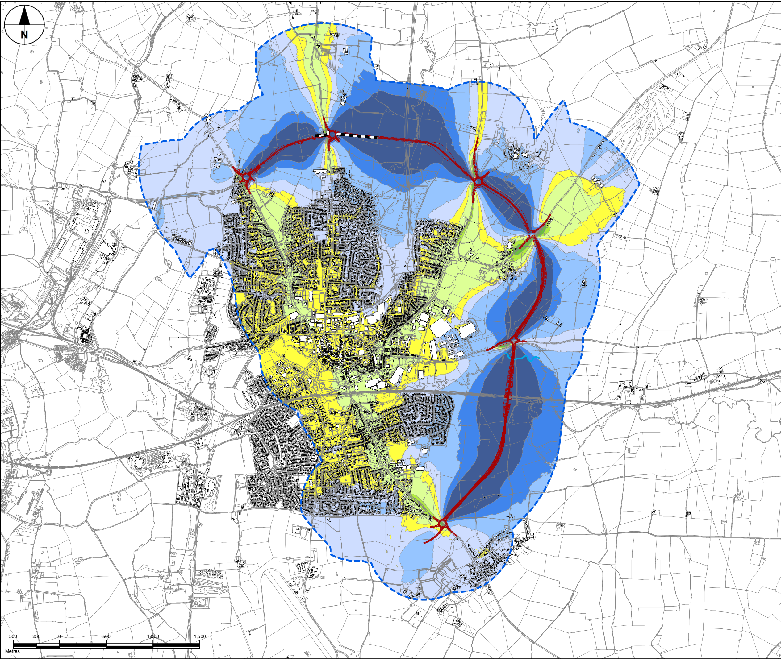
FIGURE 11.8 2021 DO-SOMETHING MINUS 2021 DO-MINIMUM: SHORT TERM CHANGE IN TRAFFIC NOISE LEVELS
